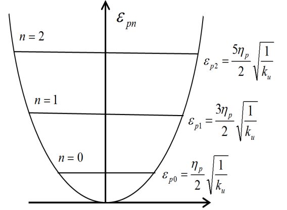
Fig. 4.1. Equidistant levels of the total mechanical energy of the \varepsilon_{pn} quantum harmonic oscillator
