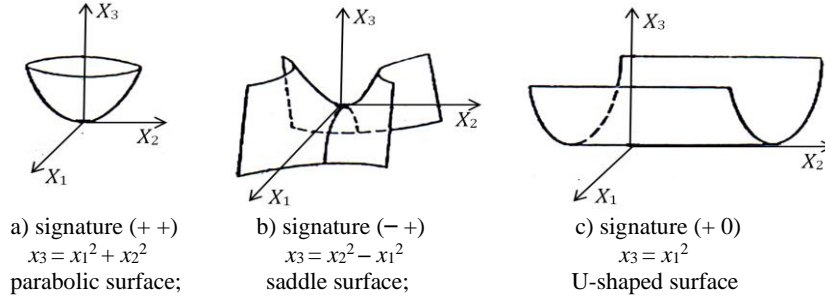
Fig. 5: Illustration of the connection between the signature of a 2-dimensional space and its topology [3]
