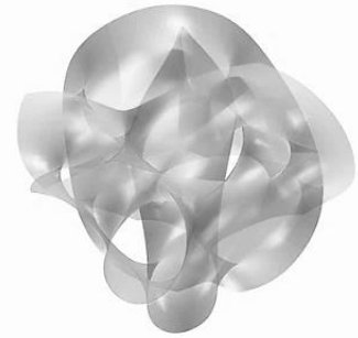
Fig. 6: One of the implementations of a 2D projection of a 3D visualization of a local area of a 10-dimensional Calabi-Yau manifold [8]
