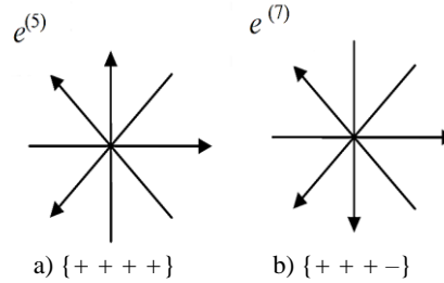
Fig. 3: Two 4-bases with different stignatures
