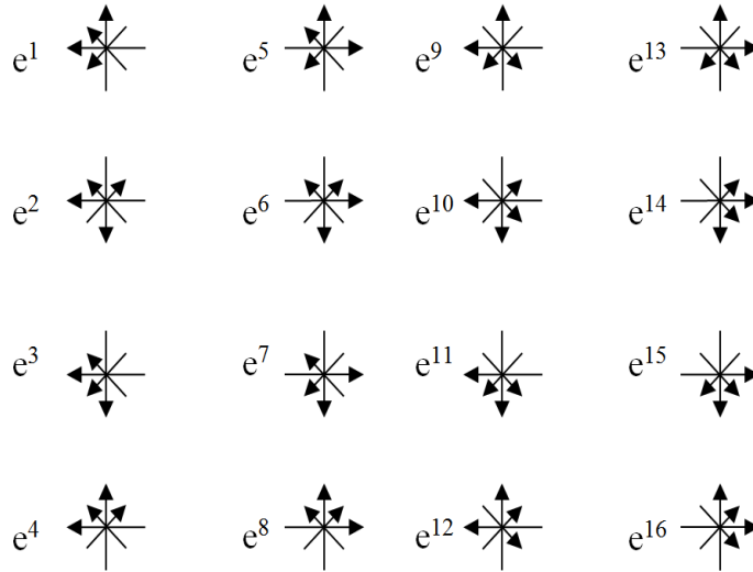
Fig. 2: Sixteen 4-bases starting at point O [1]
