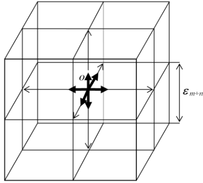
Fig. 1: Non-curved 3D light lattice of \lambda_{m,n} -vacuum, revealed from the "vacuum" (emptiness) by means of mutually perpendicular monochromatic rays of light with a wavelength \lambda_{m,n} . The cells of such a lattice are cubes with edge length \varepsilon_{m+n} \sim 10^2 \cdot \lambda_{m,n}
