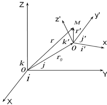
Rice. 8: Motion of the reference frame (or affine space) K' with signature \{++++\} relative the rest reference frame (or affine space) K with signature \{++++\}
