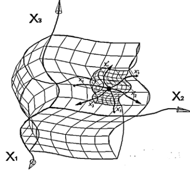
Fig. 1: \lambda_{m,n} -vacuum is embedded in \lambda_{f,d} -vacuum, where \lambda_{f,d} > \lambda_{m,n} (repetition of Figure 3 in [3])
