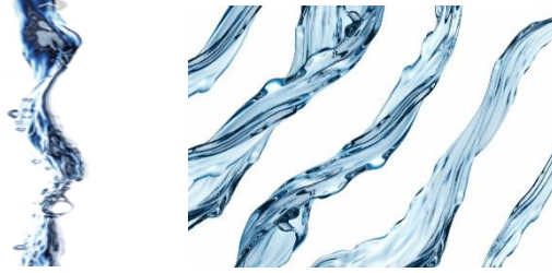
Fig. 5: Many streams in a freely falling stream of liquid twist into a spiral
