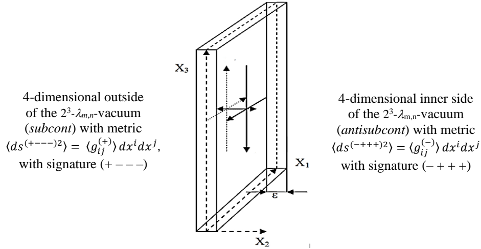
Fig. 1: Simplified illustration of a two-sided section of the 2^3 - \lambda_{m,n} -vacuum, the outer side of which ( subcont ) is described by the averaged metric \langle ds^{(+---)^2} \rangle with the signature (+---) , and its inner side ( antisubcont ) is described by the metric \langle ds^{(-+++)^2} \rangle with the opposite signature (-+++) , as \varepsilon \rightarrow 0 (repetition of Figure 7 in [3])
