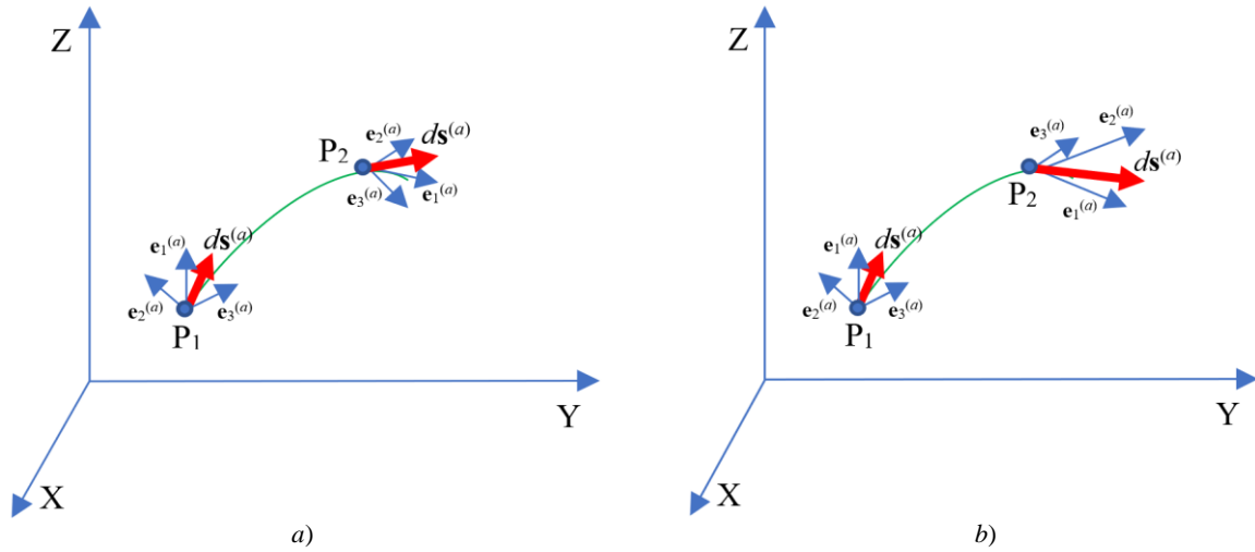
Fig. 4: a) In Riemannian geometry, the parallel translation of the vector ds^{(a)} from point p_1 to the nearby point p_2 is carried out strictly tangent to the geodesic line connecting these points. In this case, only the direction of this vector changes, and its magnitude remains unchanged. It means that the magnitude of the basis vectors \mathbf{e}_m^{(a)} and the angles between them do not change; b) In the most complexly curved, displaced and twisted space, when transferring (i.e. translation) the vector ds^{(a)} from point p_1 to the nearby point p_2 , its direction, magnitude and displacement may change. When transferring the vector ds^{(a)} in such a complexly distorted space, the magnitude of the basis vectors \mathbf{e}_m^{(a)} and the angles between them can change, and the 4-basis itself as a whole can rotate and shift. In this case, all four parameters of the 4-basis \alpha_{ij}^{(a)} , \beta^{pm(a)} , \mathbf{e}_m^{(a)} , dx^{j(a)} can change, which, according to expression (14), affects the change in the vector ds^{(a)} when it is transferred.
